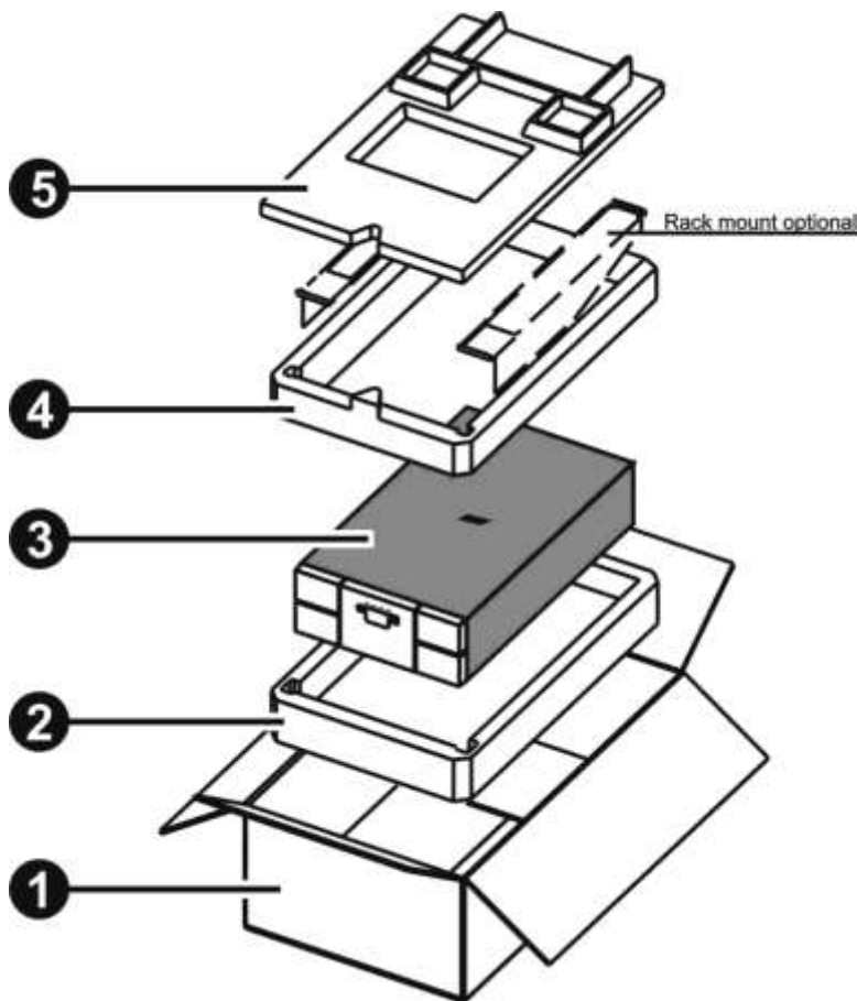
Figure 71 Packaging the Q48 library
