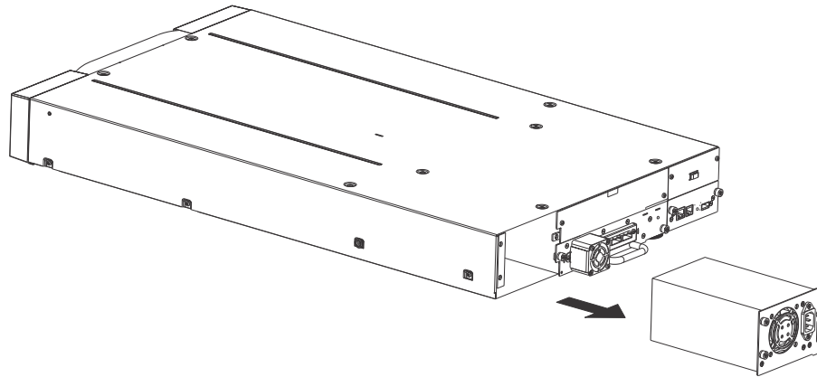
Figure 67 Remove the power supply
