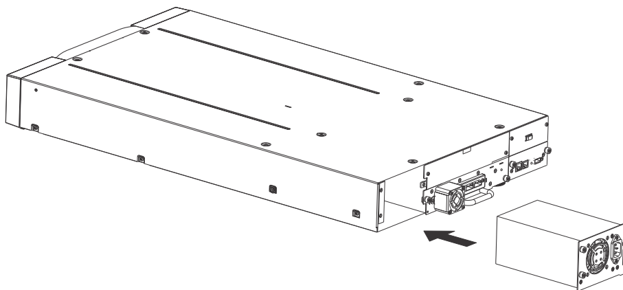
Figure 18 Install a power supply
