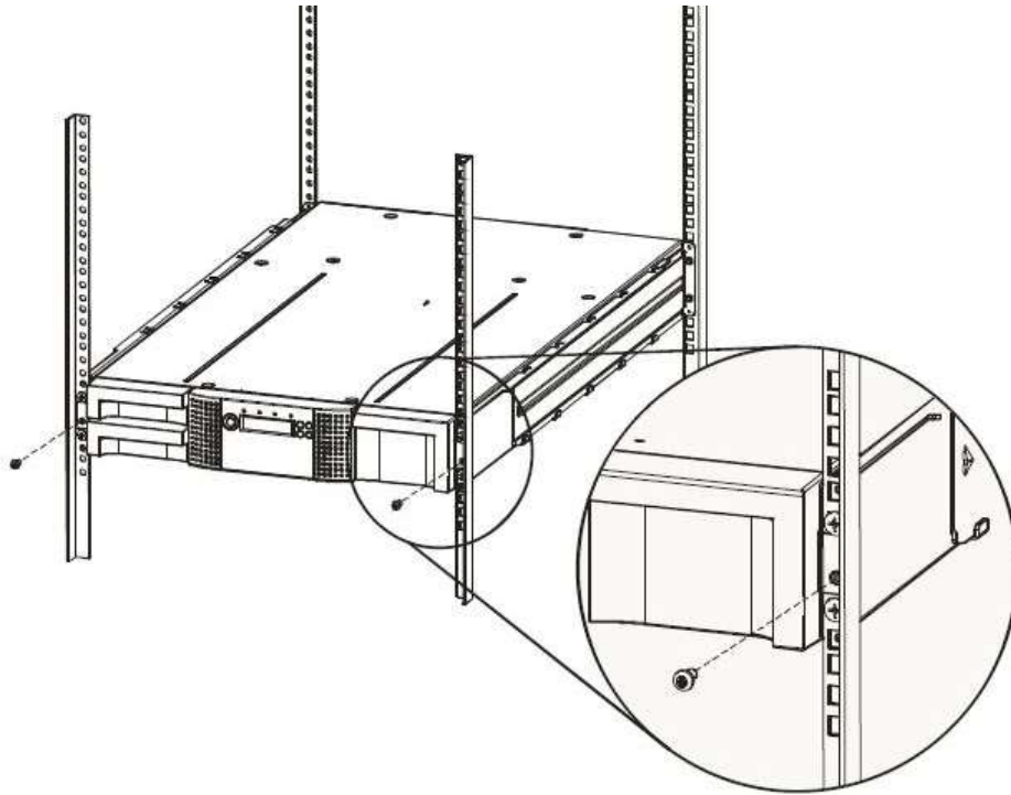
Figure 14 Secure the library to the rack
