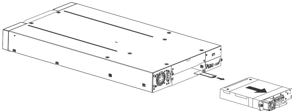
Figure 65 Remove a tape drive
