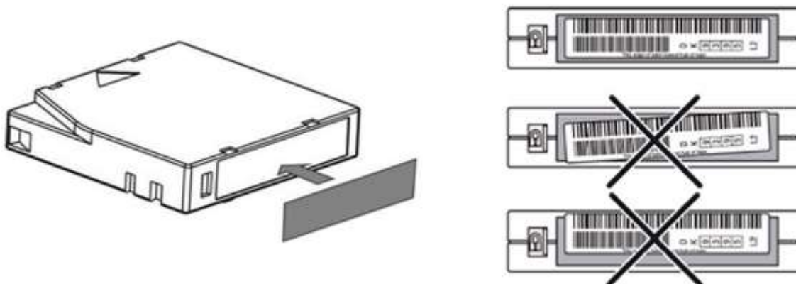
Figure 20 Proper barcode label placement
