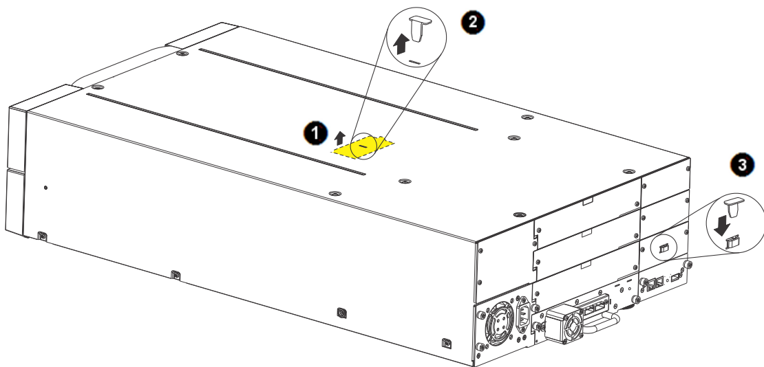
Figure 12 Removing and Storing the Shipping Lock on a Q48
