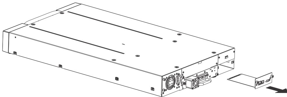
Figure 66 Remove the library controller
