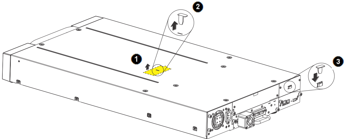
Figure 11 Removing and Storing the Shipping Lock on a Q24
