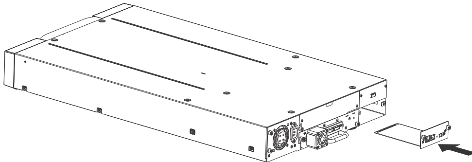
Figure 17 Install a library controller
